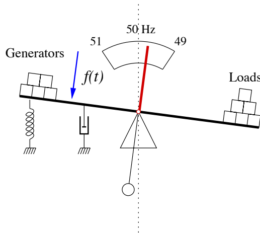
Figure 9. Renewable sources have several effects on the system: they add randomness and reduce inertia, spinning reserve and damping.
