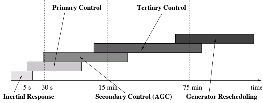
Figure 1. Typical time scales of synchronous machines and active power regulation.
