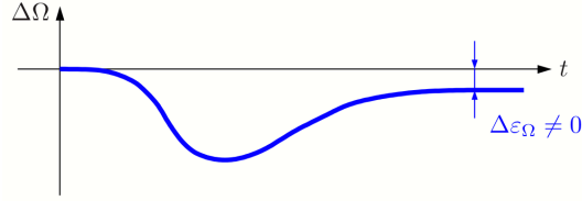
Figure 3. Typical time response of the primary frequency control after a contingency. Note that the frequency does not recover the initial value in steady-state.
