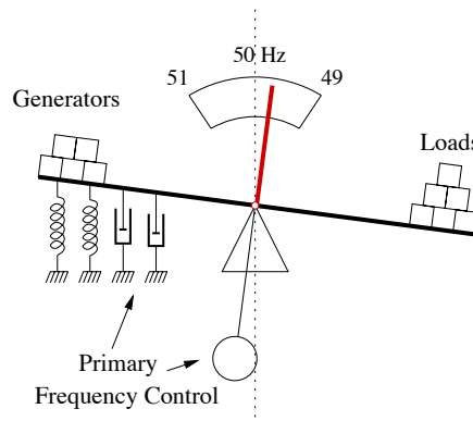
Figure 8. A low-mass center with damper represents the effect of primary frequency control.
