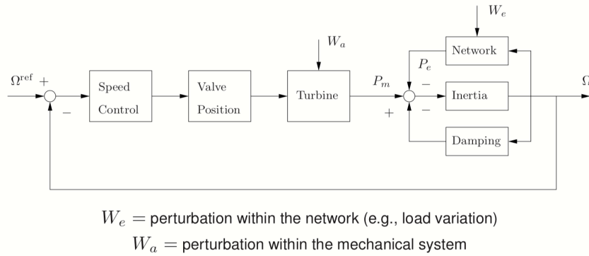
Figure 2. Typical scheme of a primary frequency controller.
