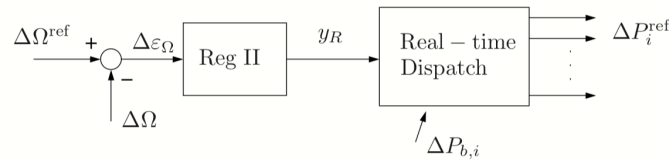
Figure 4. Typical scheme of principle of the secondary frequency control or AGC.
