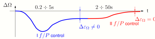
Figure 5. Typical dynamic response of the primary and secondary frequency control after a contingency. Note that the secondary frequency control is able to recover the reference frequency in steady-state.
