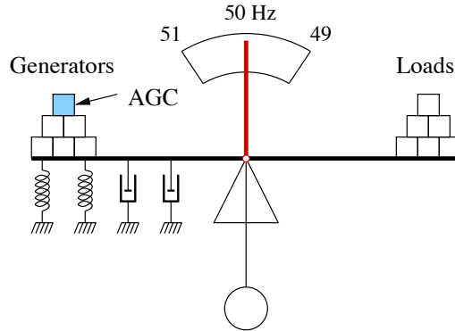
Figure 8. The AGC simply reschedules the active power set point of the machines.
