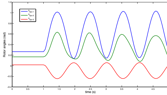
Figure 1. Typical dynamic response of uncontrolled synchronous machines after a contingency.
